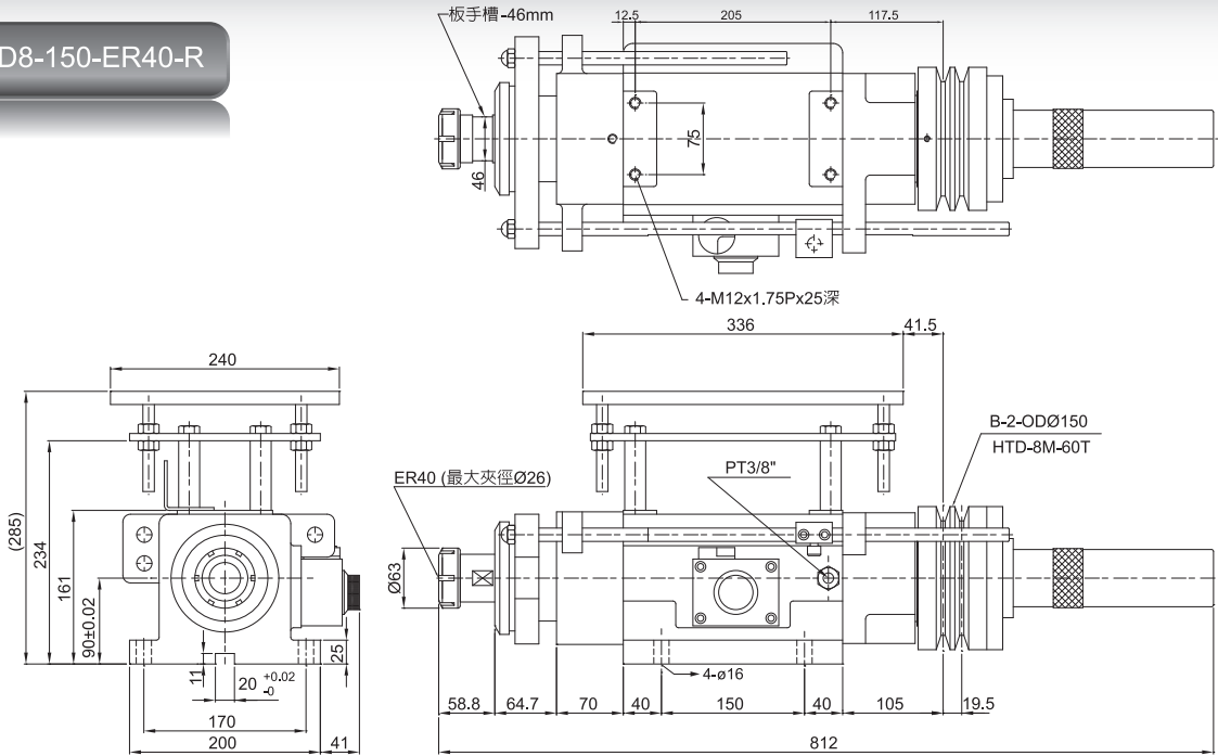
SWD8-200-ER40-R
