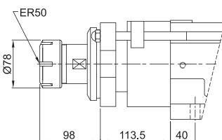
SWD8-150-ER50
