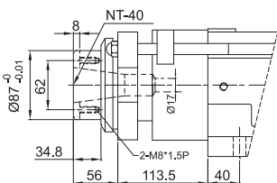
SWD8-150-NT40
