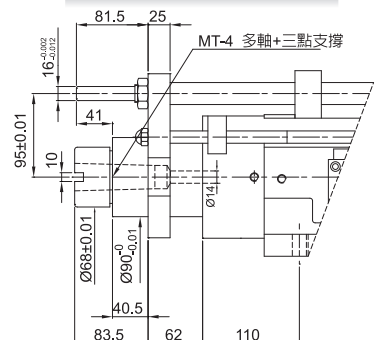
SWD8-150-MT4B-HP
