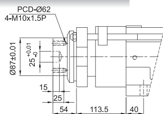
SWD8-150-FA25
